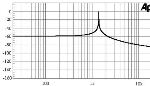
Figure 8-3 FFT of Sine Wave with No Window
