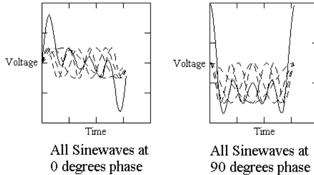
Figure 10-2 Two Multitones with Different Phases
