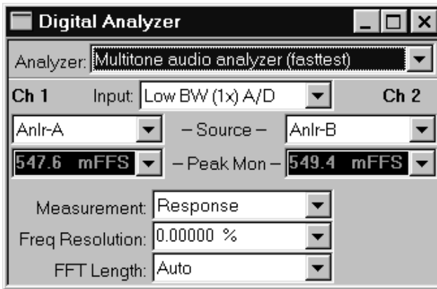
Figure 9-3 Digital Analyzer Panel for System Two
