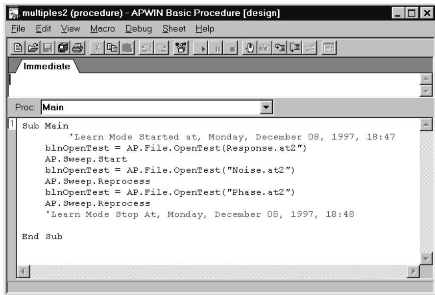
Figure 9-11 Procedure Editor After Learn
