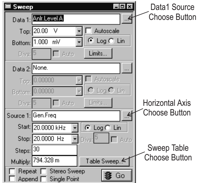
Figure 6-6 Sweep Panel, Small Version
