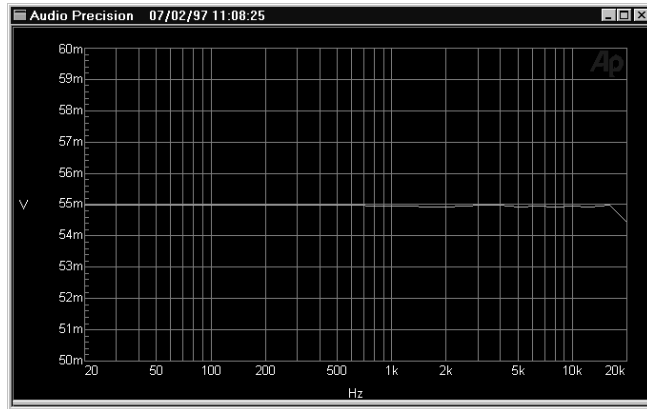
Figure 9-7 Frequency Response of System Two
