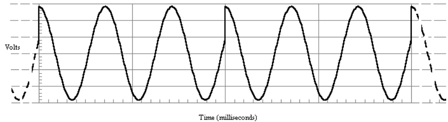
Figure 8-2 Single Sine Wave As Seen by FFT
